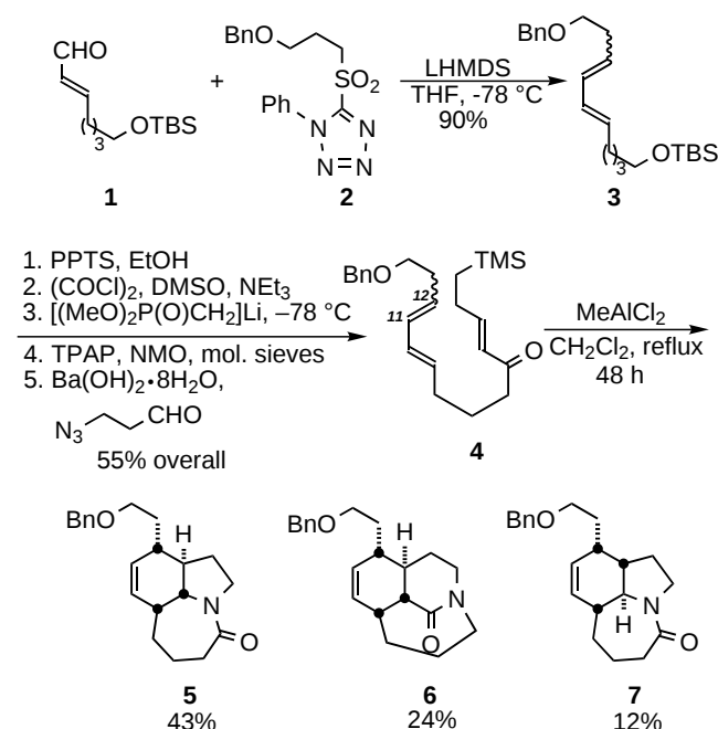
Scheme 2. Construction of the ABD-ring framework of stenine. TBS = tert -butyldimethylsilyl, LHMDS = lithium bis(trimethylsilyl)amide, PPTS = pyridinium 4-toluenesulfonate, TPAP = tetrapropylammonium perruthenate, NMO = 4-methylmorpholine N -oxide.
